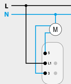
ELECTRIC BLIND PUSH BUTTON
