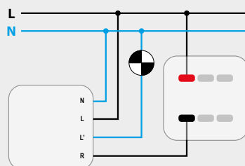
IR DETECTOR WITH PUSH BUTTON - GARBY COLONIAL (37750...), 1950 (79750...)
