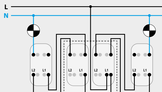
TWO-WAY SWITCH DOUBLE TWO-WAY SWITCH
