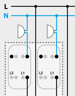
DOUBLE PUSH BUTTON
