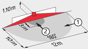
Detection area: 1) Lateral range 2) Frontal range
