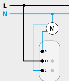
ELECTRIC BLIND SWITCH
