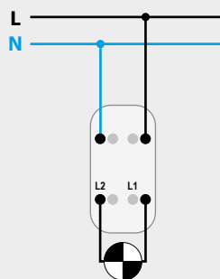
DOUBLE-POLE SWITCH
