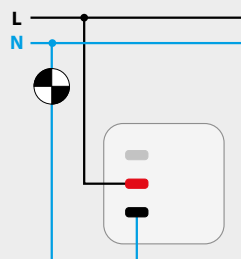
HOTEL CARD SWITCH, 1 MICROSWITCH - GARBY COLONIAL (37935...)
