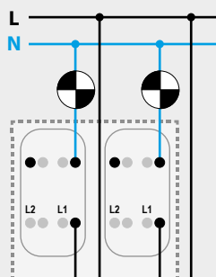
DOUBLE ONE-WAY SWITCH
