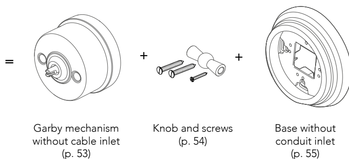
With universal flush-mounted box and base
