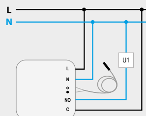
CONNECTED THERMOSTAT - 1950 (79731...) + SENSOR (7973200)
