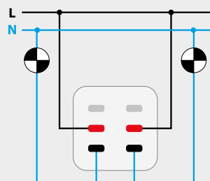
HOTEL CARD SWITCH, 2 MICROSWITCHES - GARBY COLONIAL (37936...)
