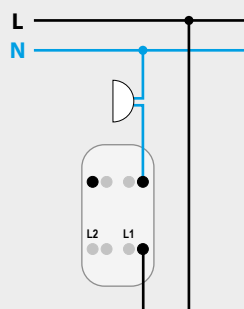
PUSH BUTTON
