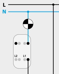
ONE-WAY SWITCH
