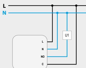
THERMOSTAT - 1950 (797300...)
