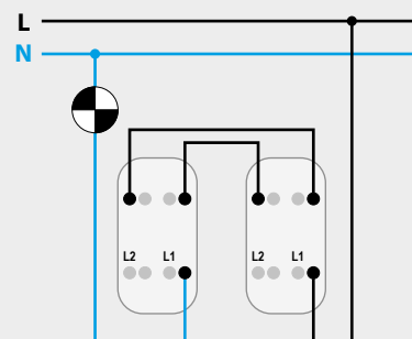
TWO-WAY SWITCH
