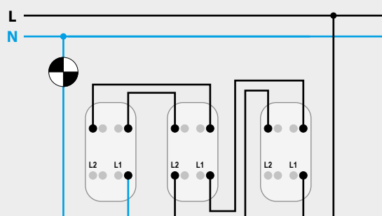
TWO-WAY SWITCH INTERMEDIATE SWITCH
